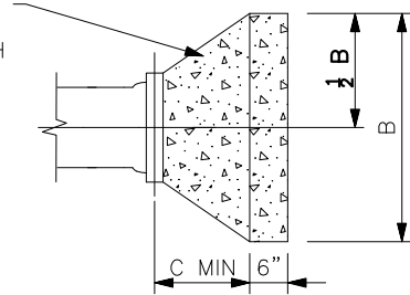
SEC X-X
